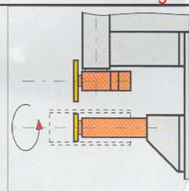
Transversal welding
