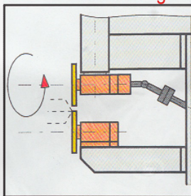
Transversal welding
